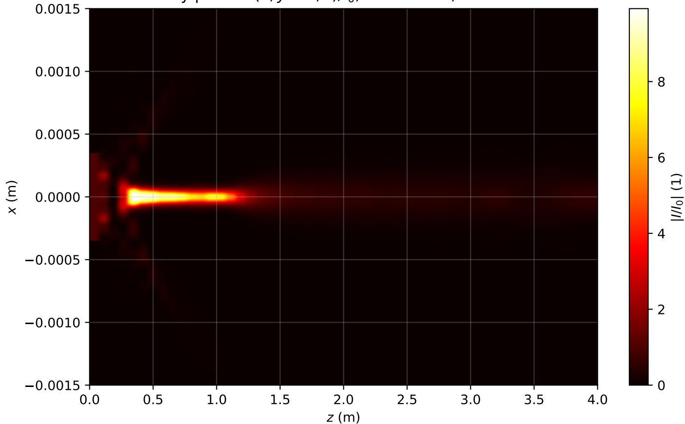
Intensity profile I(x, y = 0, z)/I_0 , P_{in}=7.0P_{cr} , artificial time
